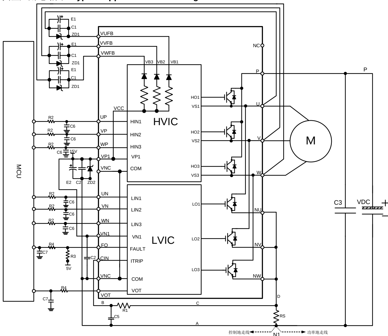
典型应用电路图 Typical application circuit diagram
