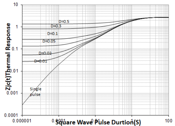
Transient Thermal Response Curve For MS65R135R/TO-247
