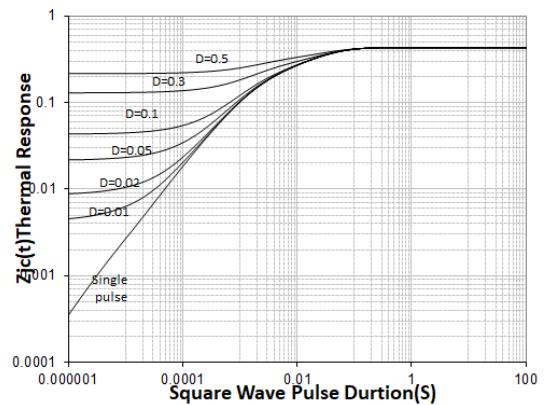
Transient Thermal Response Curve For MS65R135R/TO-247
