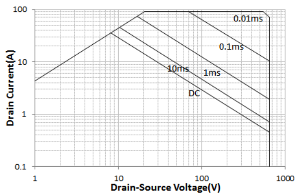
Maximum Safe Operating Area For MS65R135R/TO-247
